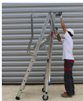
Pull the bracket plane down by lowering the floor
