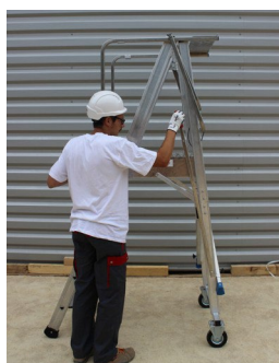
Installation of the handles (2 hexagon socket screws at the ends of each handle, 4 in total + an Allen key)
